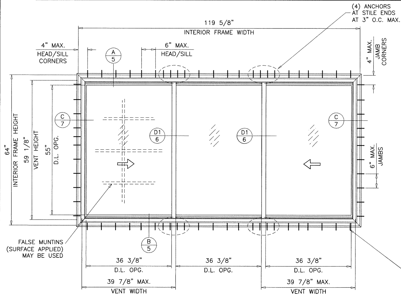
FLANGE FRAMES
